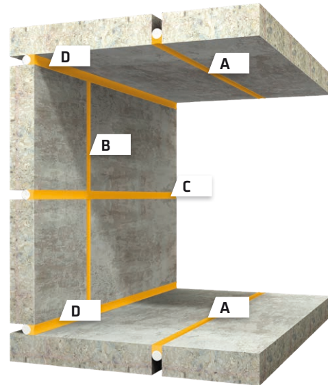
Horizontal floor joint abutting a wall.
