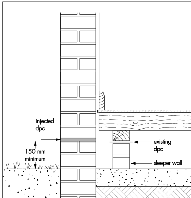
Figure 1 Suspended timber floor on sleeper wall
