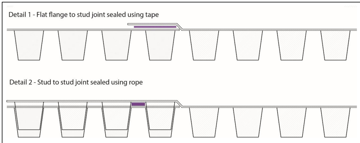
Figure 3 Sika Jointing Tape and Sika Rope sealing
