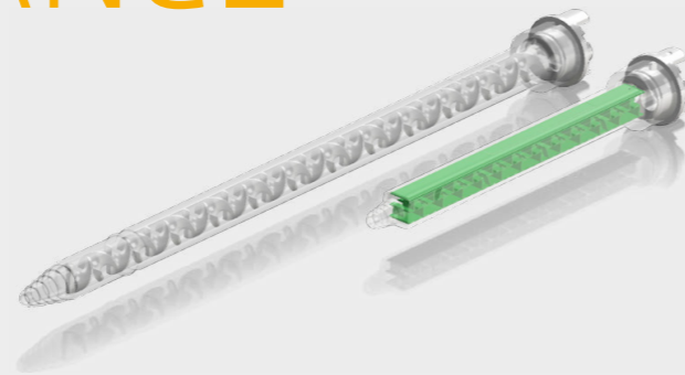
Equivalent sized mixers. Helix mixer (LHS) and Quadro mixer (RHS)
