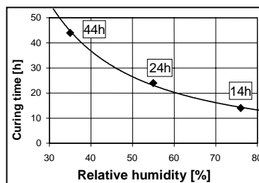
Curing time for 500 µm adhesive film 3) at 20°C
