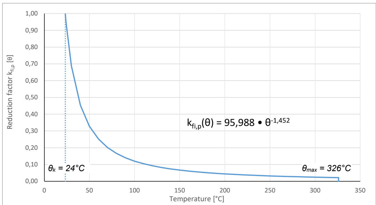
Figure C1: Reduction factor k_{fi,p}(\theta)
