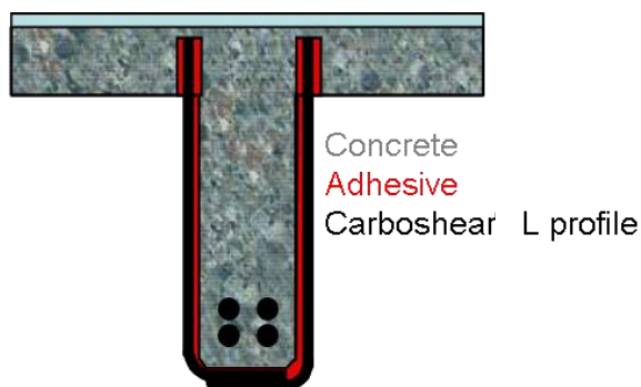
Sika® CarboShear for shear strengthening
