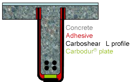
Sika® CarboShear for shear strengthening and improved end anchorage of Sika® CarboDur® Plates
