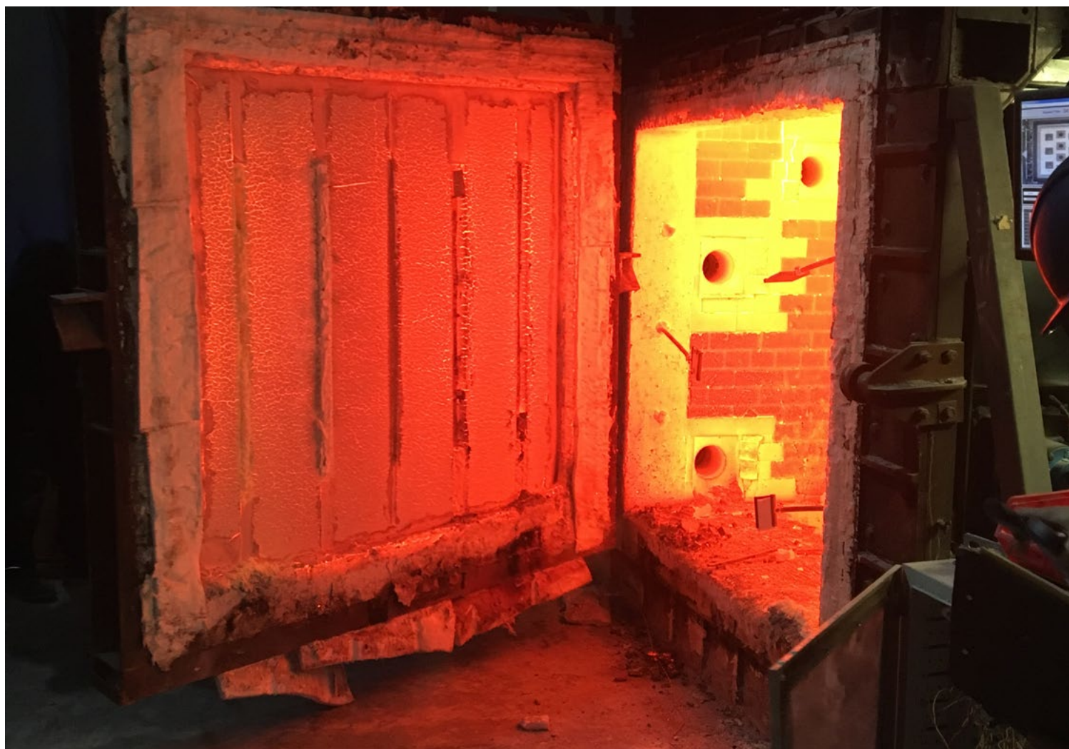
Furnace with vertical linear seals after resistance to fire test acc. EN 1366-4.
