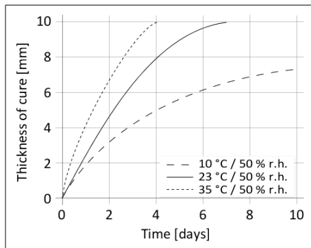
Diagram: curing speed Sikaflex®-276 PC-2
