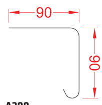
A200 STANDARD DRIP TRIM 904241
