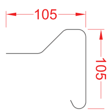
B230 SMALL RAISED EDGE TRIM 903751
