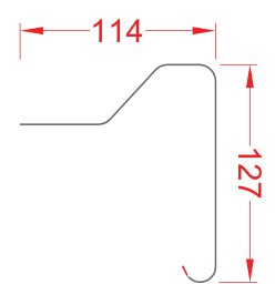
B260 STANDARD RAISED EDGE TRIM 902825
