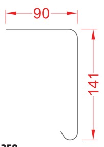
A250 LARGE DRIP TRIM 909988
