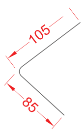
EXT 195 EXTERNAL RAISED ANGLE TRIM 909987
