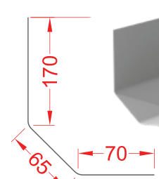
D300 WALL FILLET TRIM 904759
