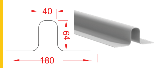
E180 EXPANSION JOINT / ROLL MOP TRIM 902703
