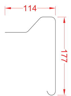
B300 LARGE RAISED EDGE TRIM 904165
