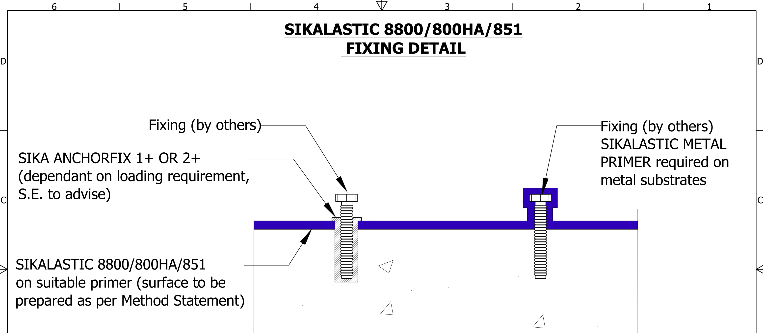
OPTION 1 POST FIXED DETAIL
