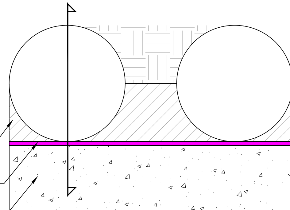
CONTIGUOUS PILE PLAN
