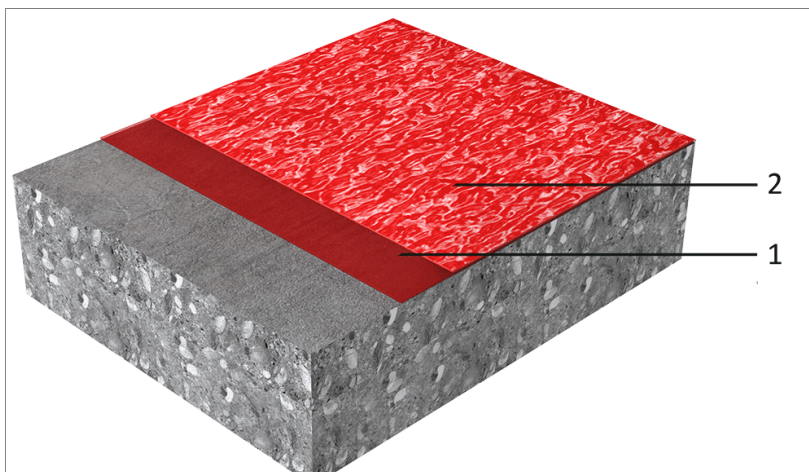
Sikafloor® MultiDur WT-10 system (~ 0.4-0.6 mm)
