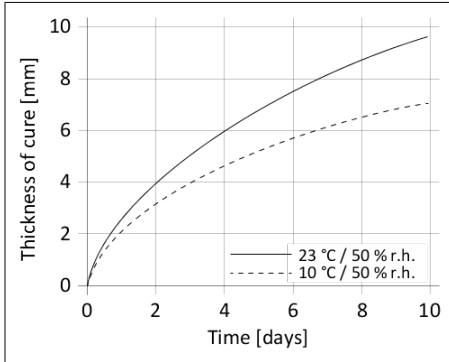
Diagram 1: Curing speed Sikaflex®-508
