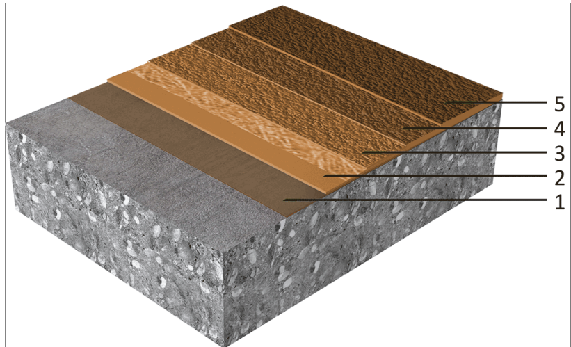
Sikafloor® Pronto RB-55 system (~4–6 mm) / Application on surfaces with inclination
