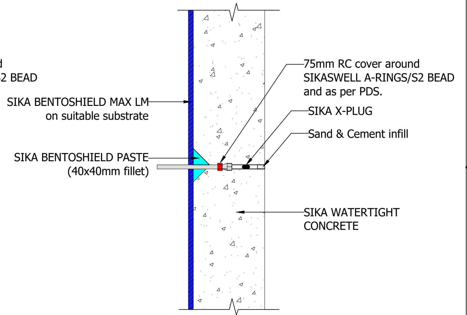
COMPLETED DETAIL
