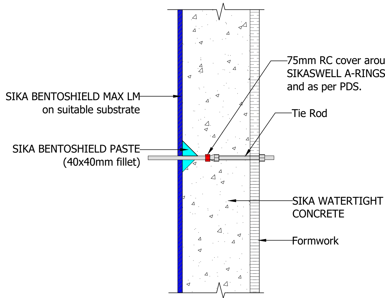
AS CONSTRUCTED
