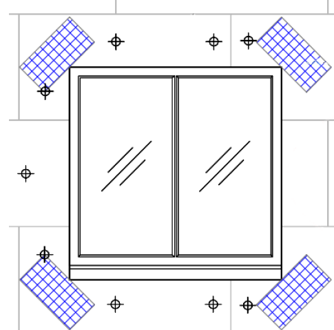
Diagram 8 - Typical opening stress patch detail
