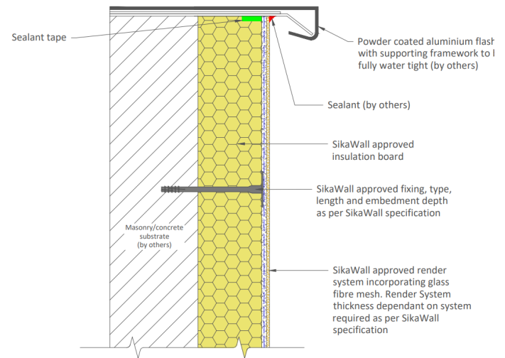
Diagram 10 - Parapet detail
