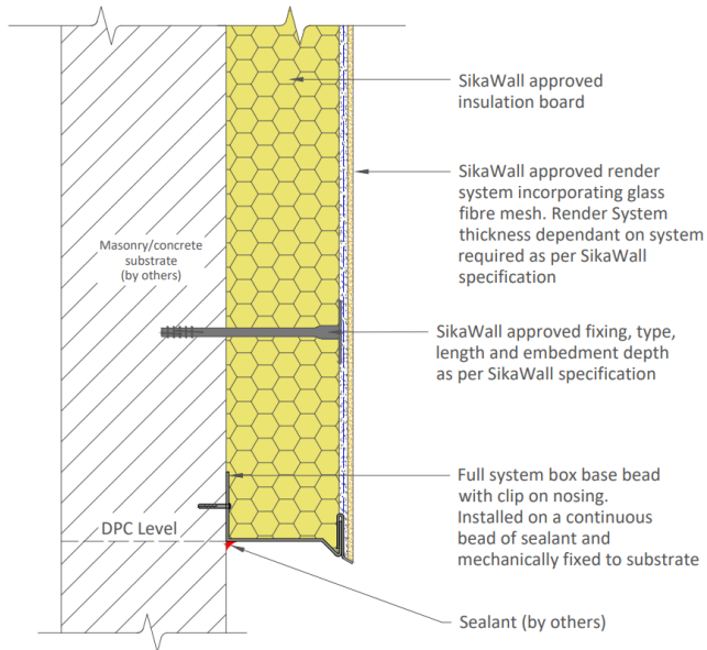
Diagram 3 - Typical standard base detail
