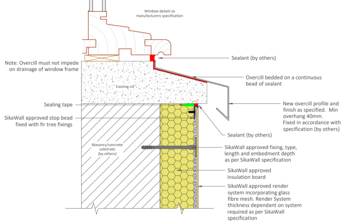
Diagram 7 - Typical over cill detail
