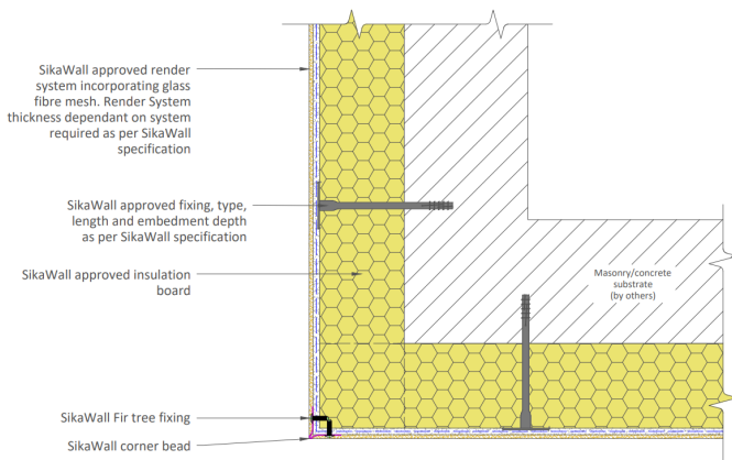
Diagram 5 - Typical external corner detail
