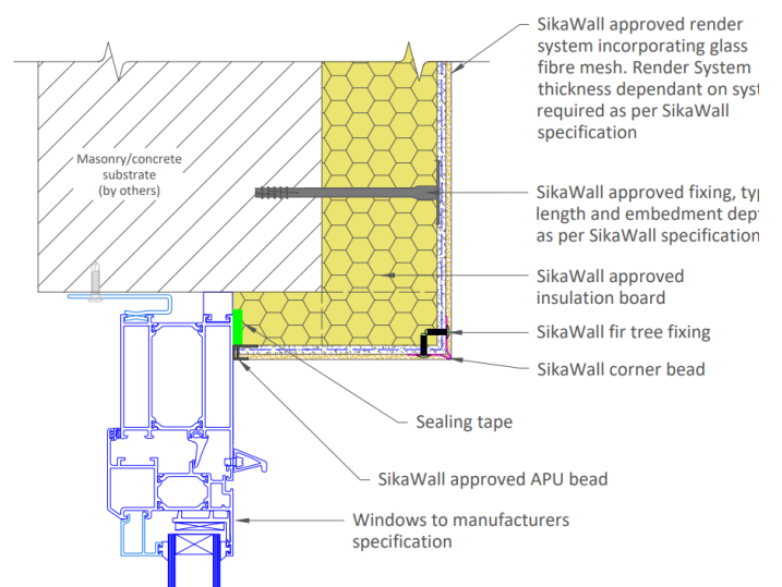
Diagram 6 - Typical window reveal/head detail
